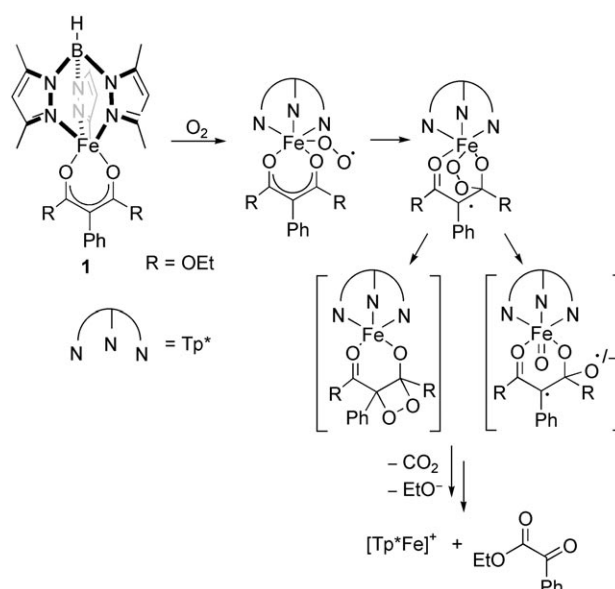
Scheme 3. Conceivable mechanism for the oxidative cleavage of diethyl phenylmalonate.
