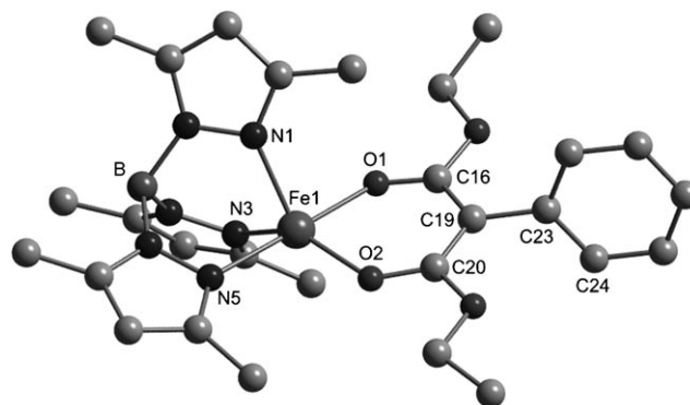
Figure 1. Molecular structure of 1 . All hydrogen atoms were omitted for clarity. Selected bond lengths [Å] and angles [°]: Fe1–O1 = 2.0876(8), Fe1–O2 = 1.9868(9), Fe1–N1 = 2.0968(11), Fe1–N3 = 2.0906(11), Fe1–N5 = 2.1678(10), O2–C20 = 1.2695(14), O1–C16 = 1.2444(15), C16–C19 = 1.4188(17), C19–C20 = 1.4026(16); C16–C19–C20 = 118.74(11), O2–Fe1–N3 = 142.34(4), O1–Fe1–N5 = 177.13(4), C16–C19–C23–C24 = 71.99(16).
