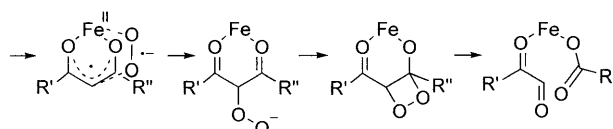
Scheme 1. Proposed mechanism for the cleavage of \beta -dicarbonyl compounds promoted by acetylacetonate dioxygenase. [4]
